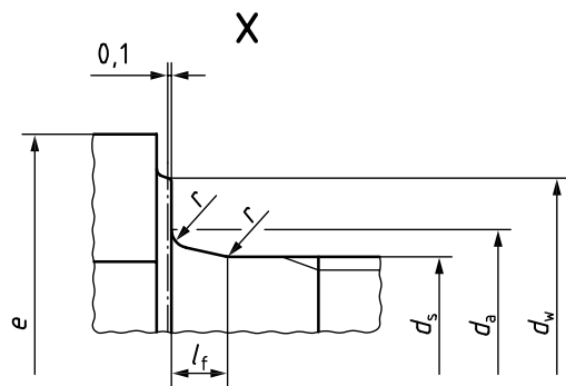
c) Full shank with conical transition
