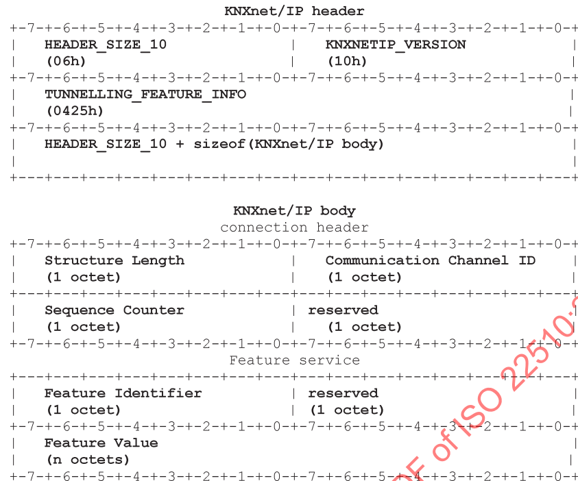
Figure 56 — TUNNELLING_FEATURE_INFO frame binary format
