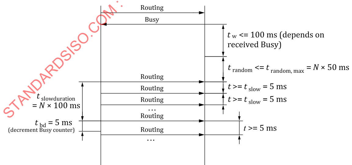
Figure 64 — Flow control with ROUTING_BUSY
