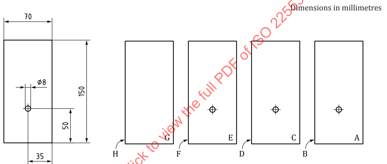
Figure 7 — Test panels
