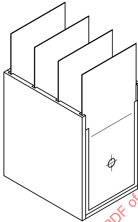
Figure 10 — Test specimen
