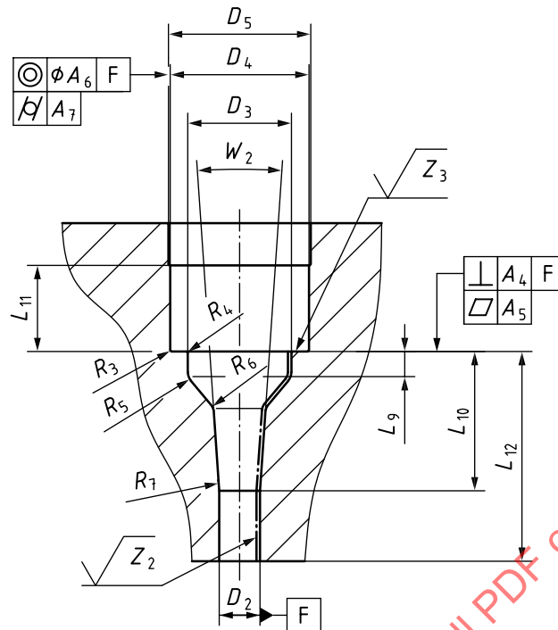
Figure 4 — Cylinder head bore
