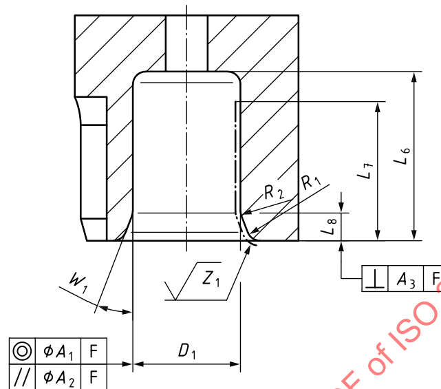
Figure 3 — Injector cup bore
