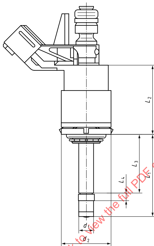
Figure 1 — Injector dimensions
