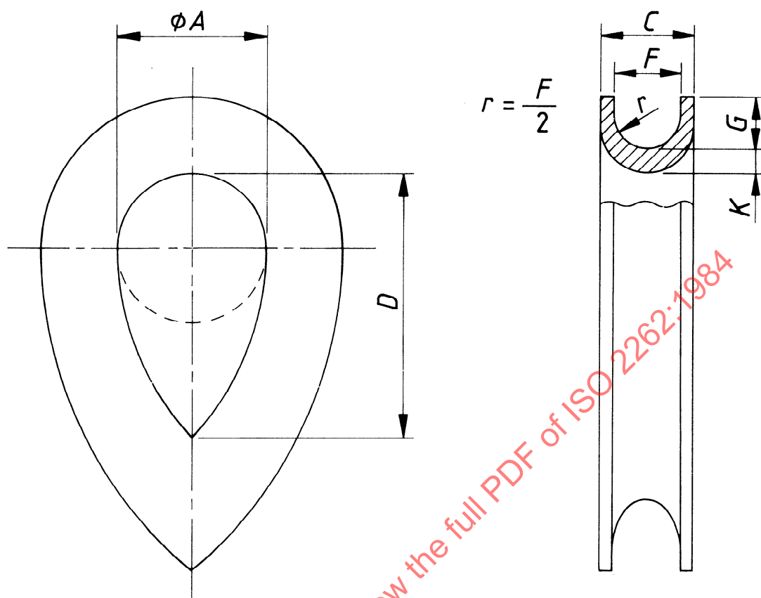
Figure 1 — Thimble with point
