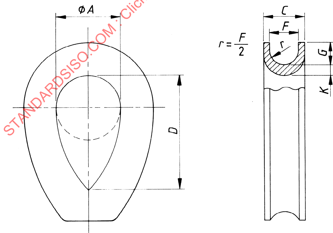
Figure 2 — Thimble without point
