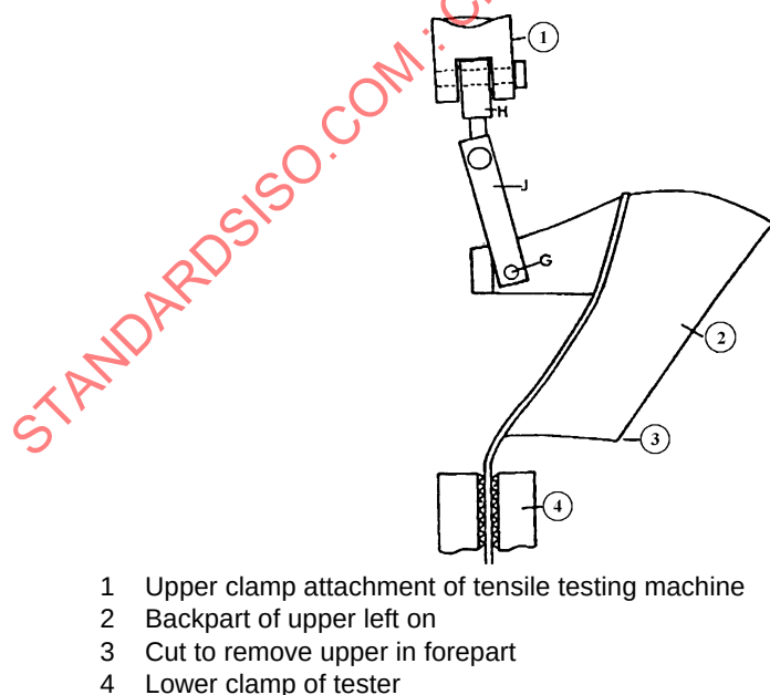
Figure 4 – Side view of shoe with chunky heel clamped in a tensile testing machine using the link shown in figure 1
