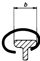
FIGURE 2 – EL traveller on ring flange
