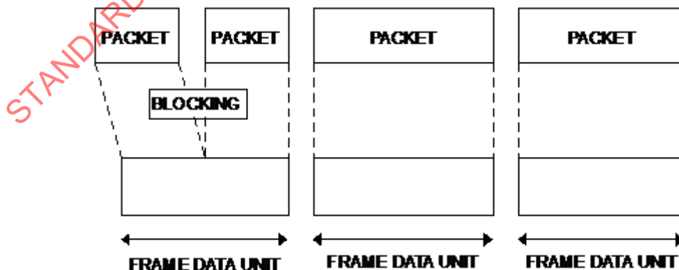
Figure 4-14: Example of VC Packet Processing Procedures
