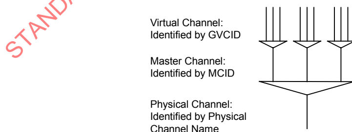
Figure 2-2: Relationships between Channels
