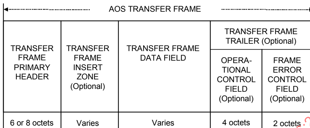
Figure 4-1: AOS Transfer Frame Structural Components
