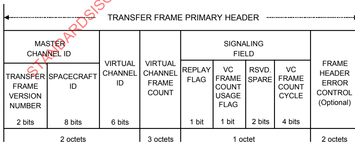
Figure 4-2: Transfer Frame Primary Header
