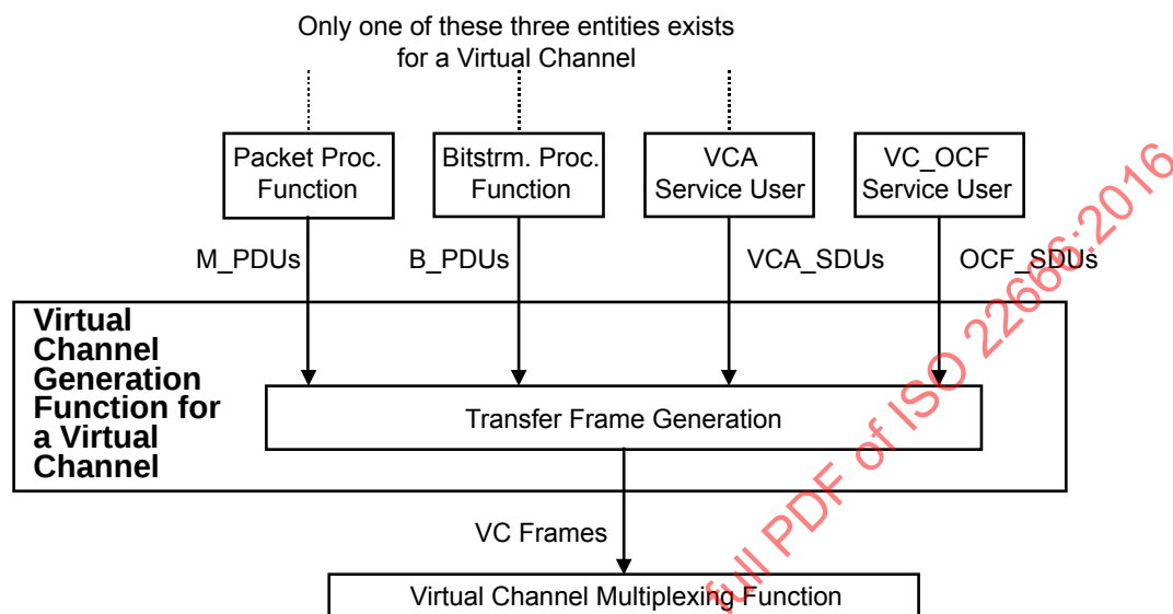
Figure 4-10: Abstract Model of Virtual Channel Generation Function
