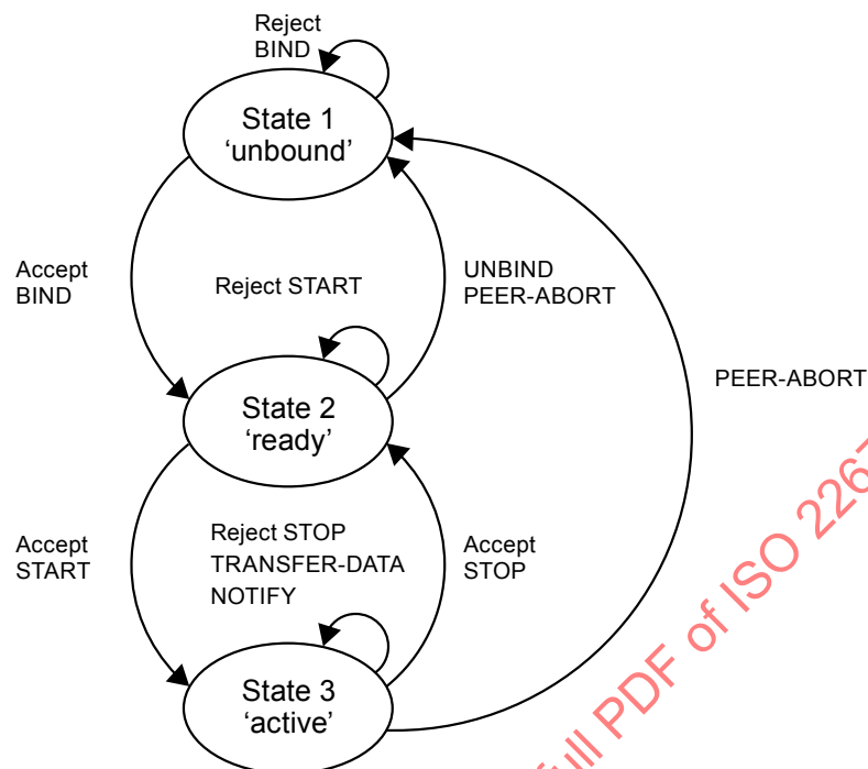
Figure 2-4: Simplified RCF Service Provider State Transition Diagram
