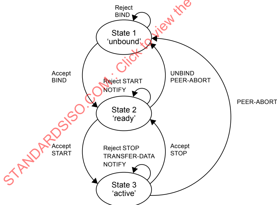
Figure 2-4: Simplified Forward CLTU Service Provider State Transition Diagram
