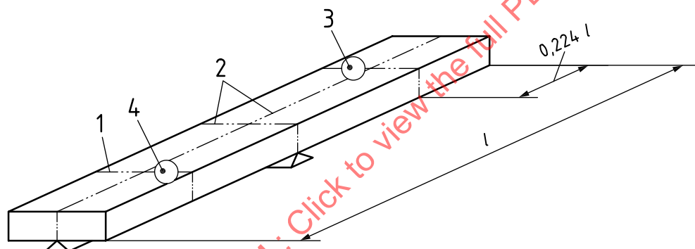
Figure 6 — Specimen oriented on the support for flexural vibration
