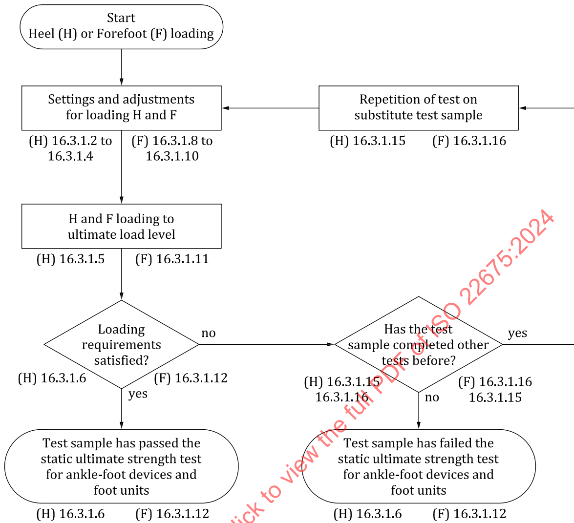
Figure 12 — Flowchart for the static ultimate strength test specified in 16.3.1
