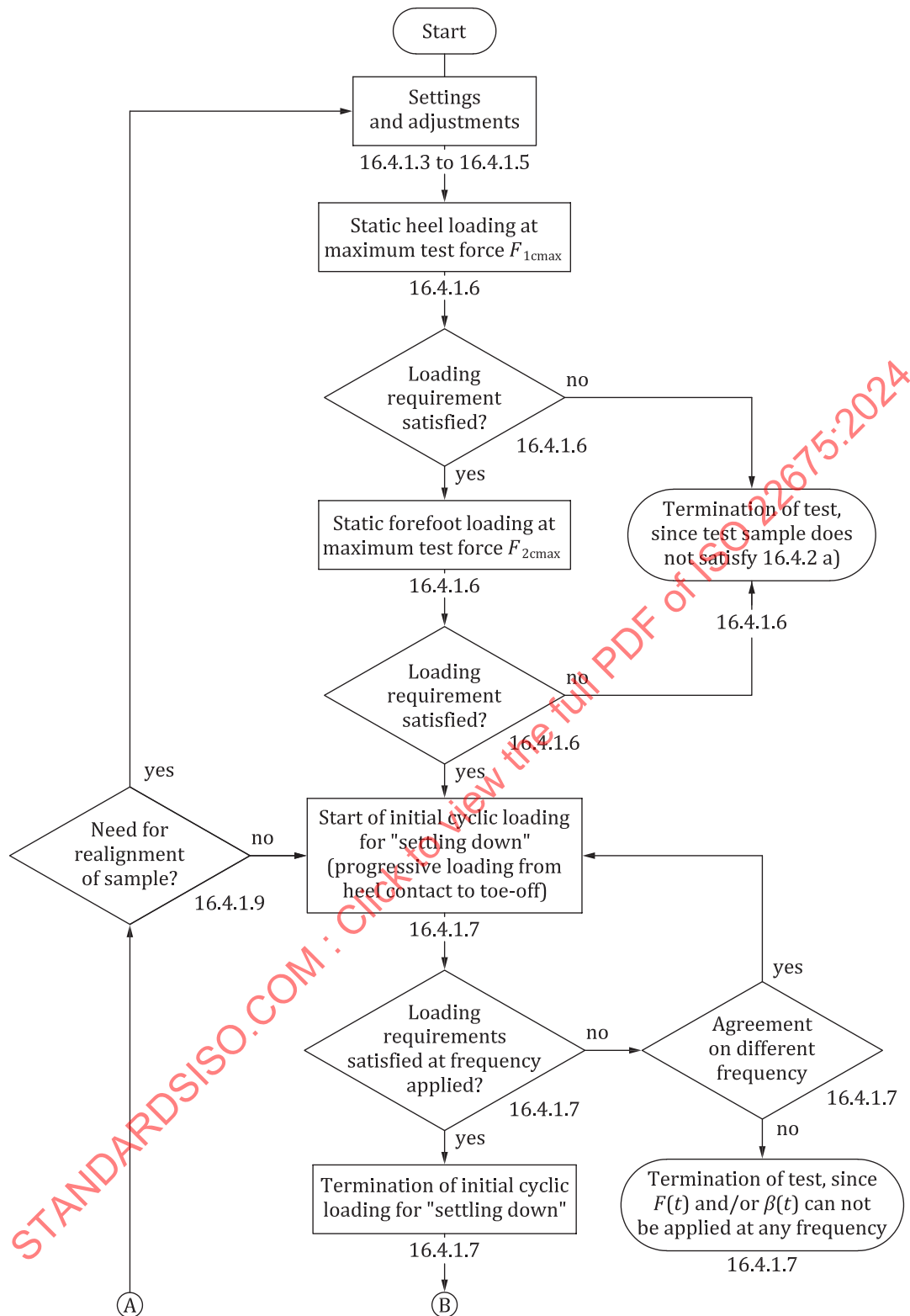
a) Flowchart for the cyclic test specified in 16.4.1 to allow the test sample and the test equipment to “settle down”.
