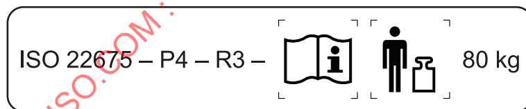
Figure 15 — Identifier layout
