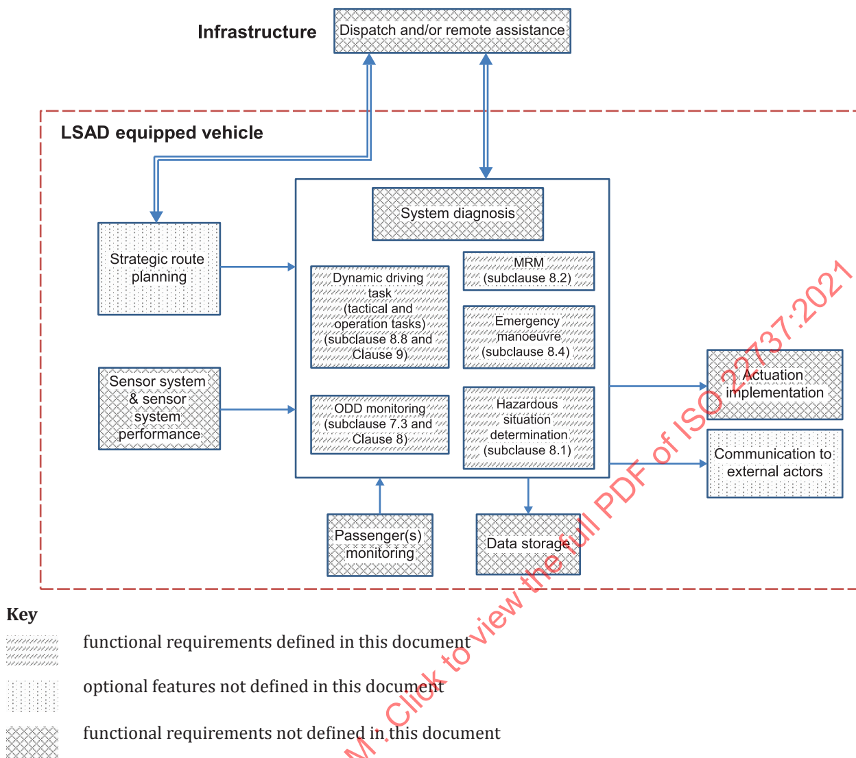
Figure 2 — Example system architecture — Individual LSAD system
