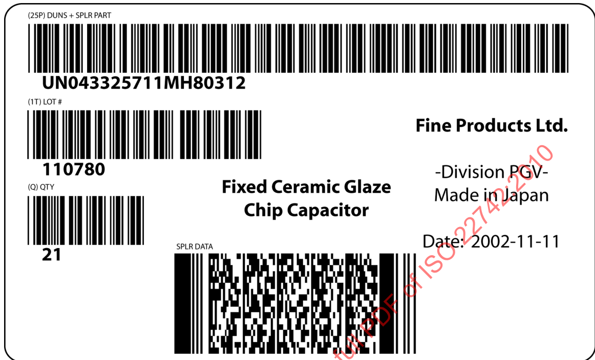
Figure 11 — Example of linear bar code symbols and PDF417 with DIs (not to scale)
