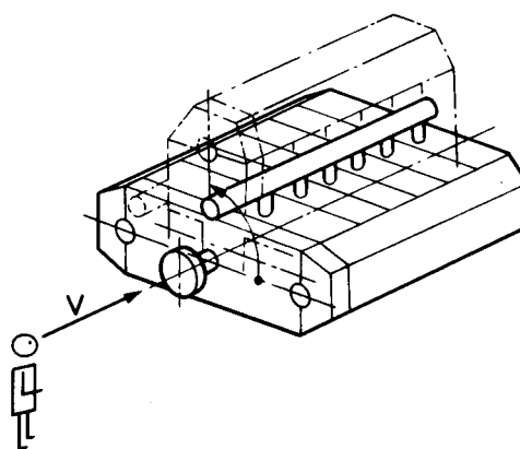
FIGURE 3f — Left-hand single bank opposed piston engine
