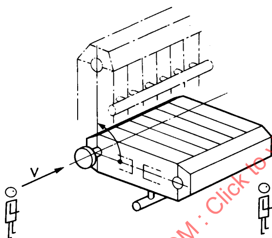
FIGURE 3c — Right-hand single bank opposed piston engine
