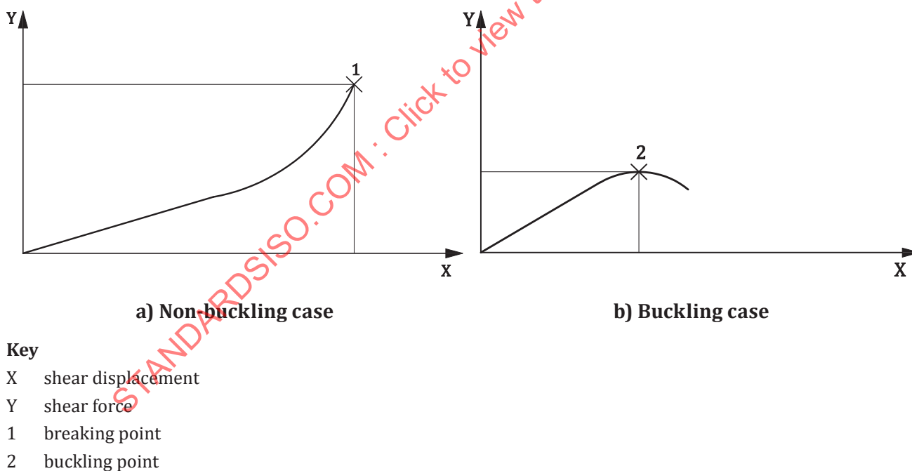
Figure 12 — Ultimate shear properties
