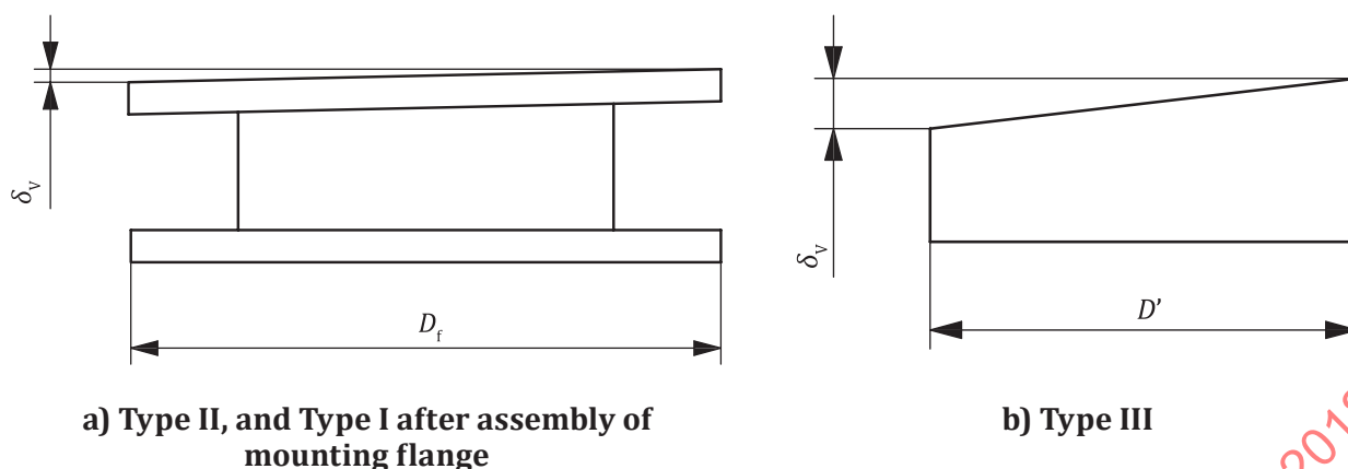
Figure 5 — Measurement of flatness
