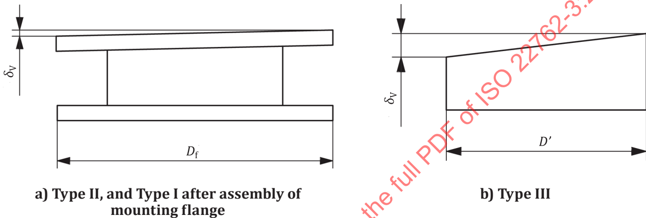
Figure 5 — Measurement of flatness
