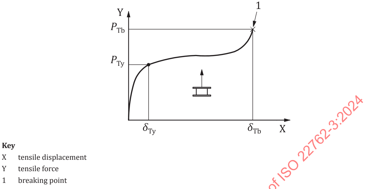
Figure 2 — Tensile properties of elastomeric isolators
