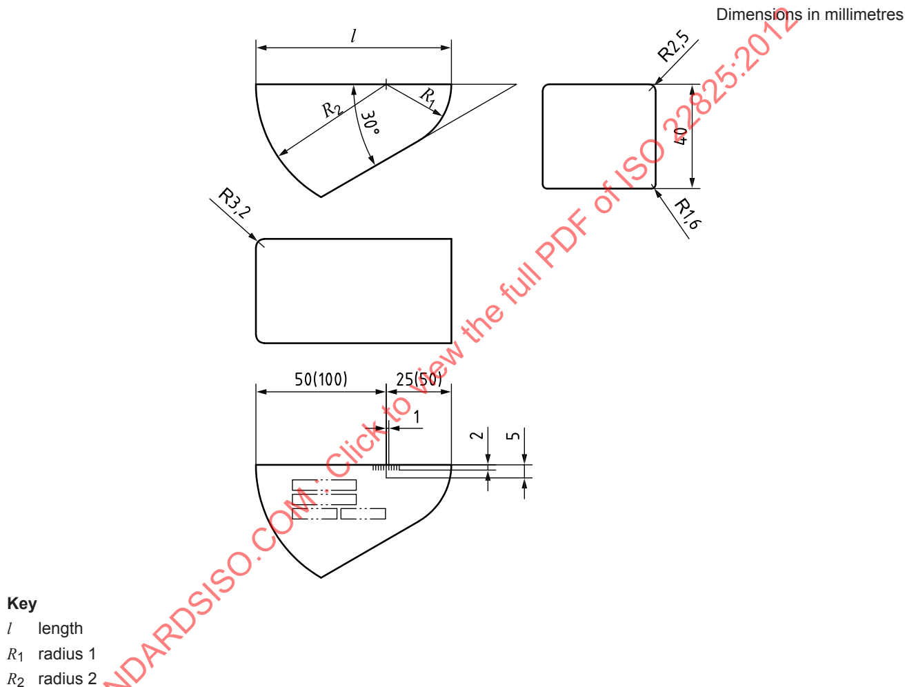
Figure B.1 — Stainless steel calibration blocks
