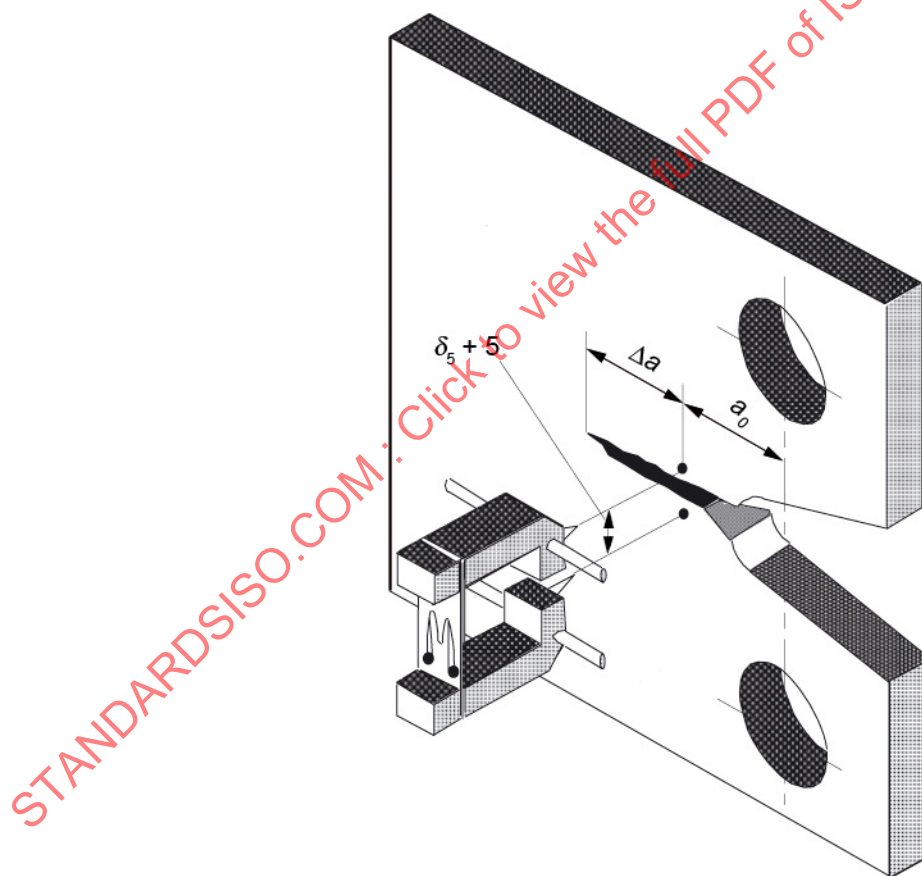
Figure B.1 — Basic arrangement for measuring \delta_5
