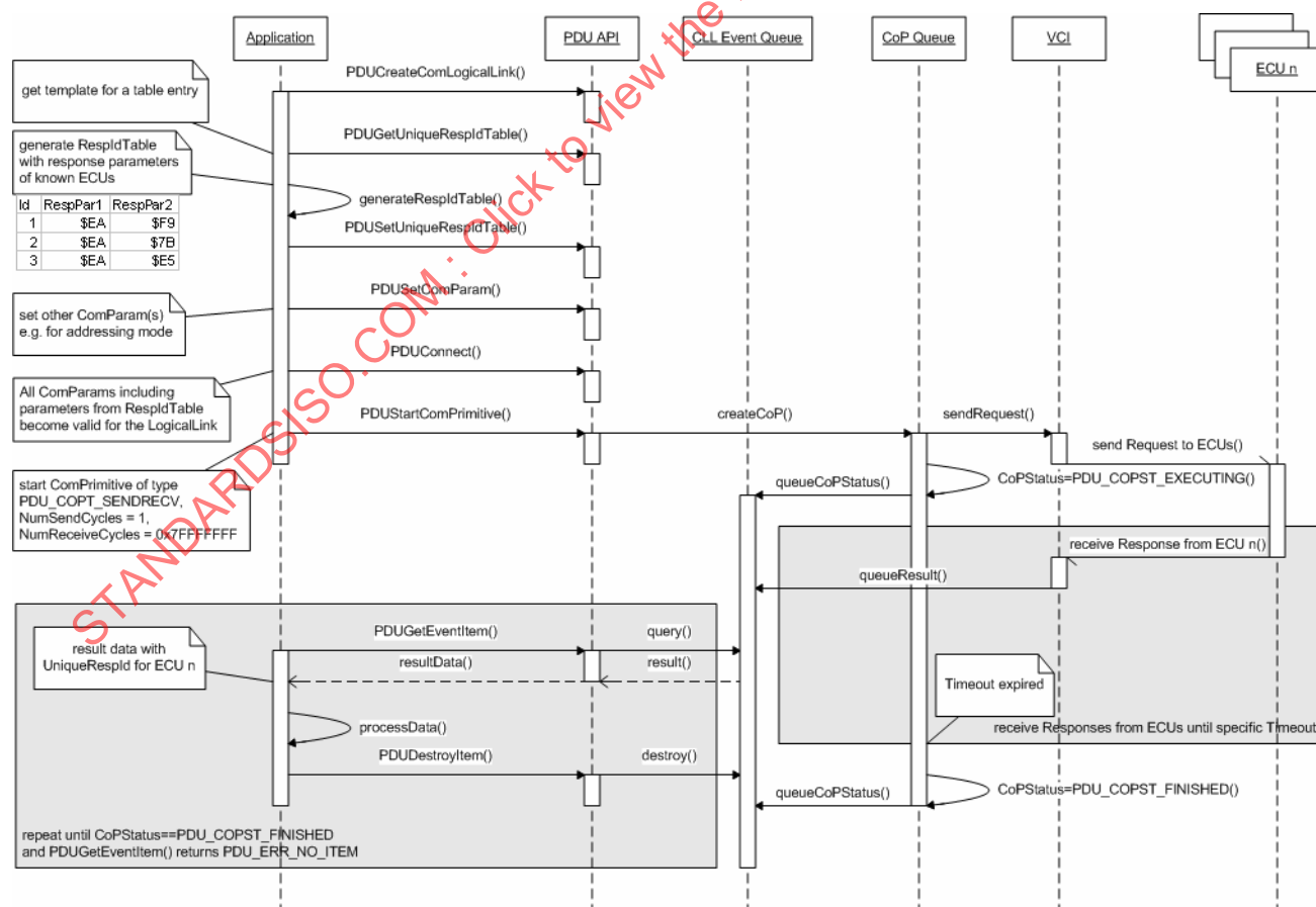
Figure 25 — Sequence of Unique Response ID Table (URID Table) for physical and functional addressing
