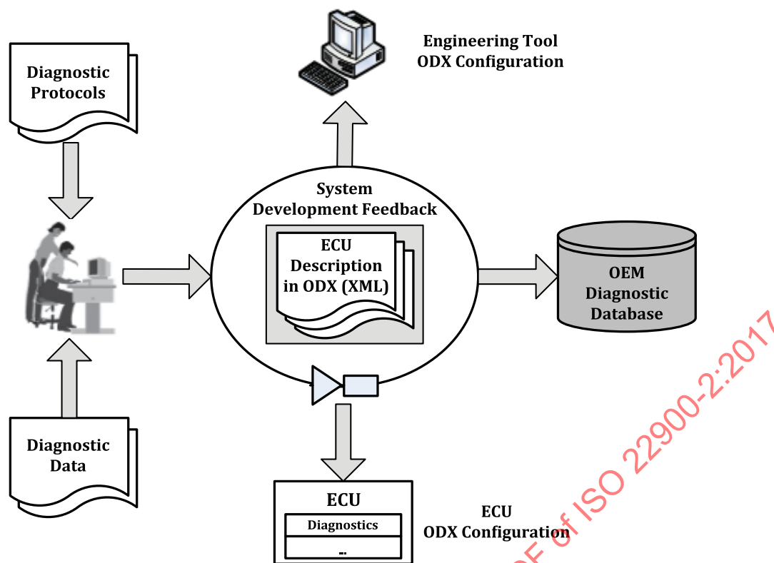
Figure 1 — Example of central source engineering diagnostic data process
