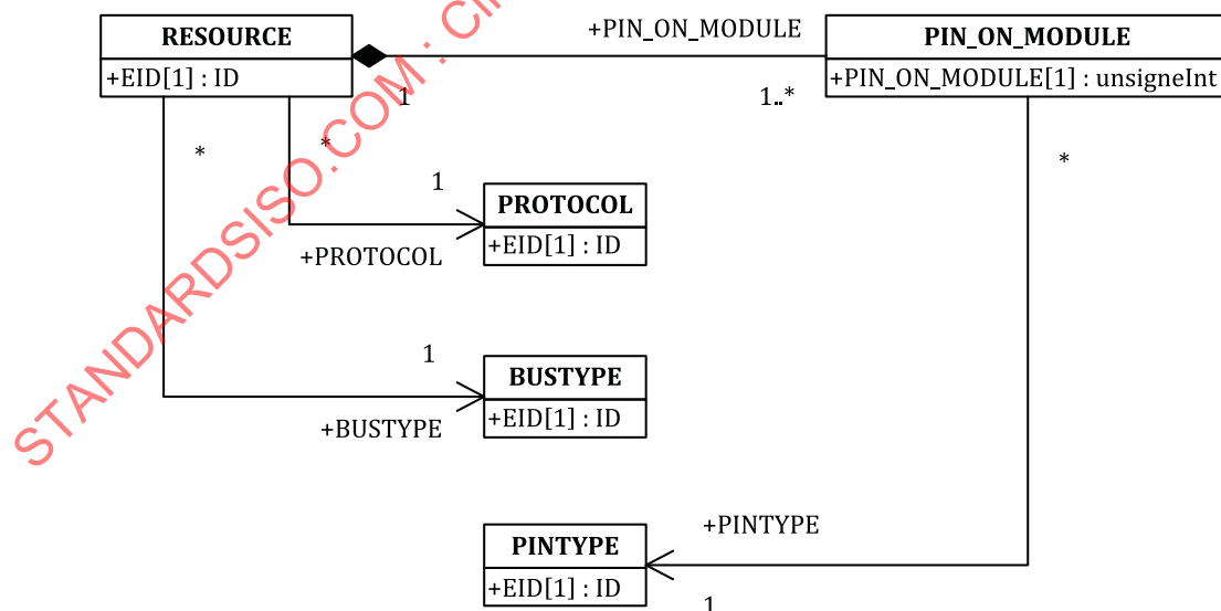
Figure F.4 — UML class diagram of element RESOURCE
