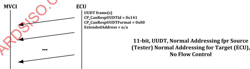
Figure B.2 — Example #1 CAN Id format configurations
