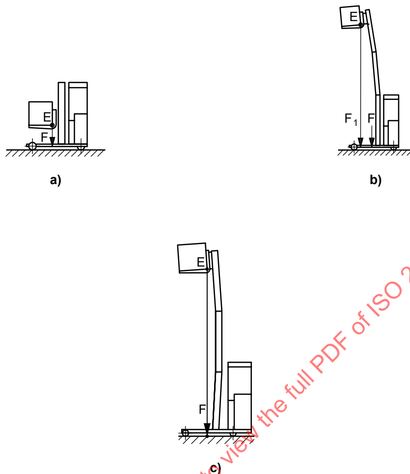
Figure 2 — Datum point positions
