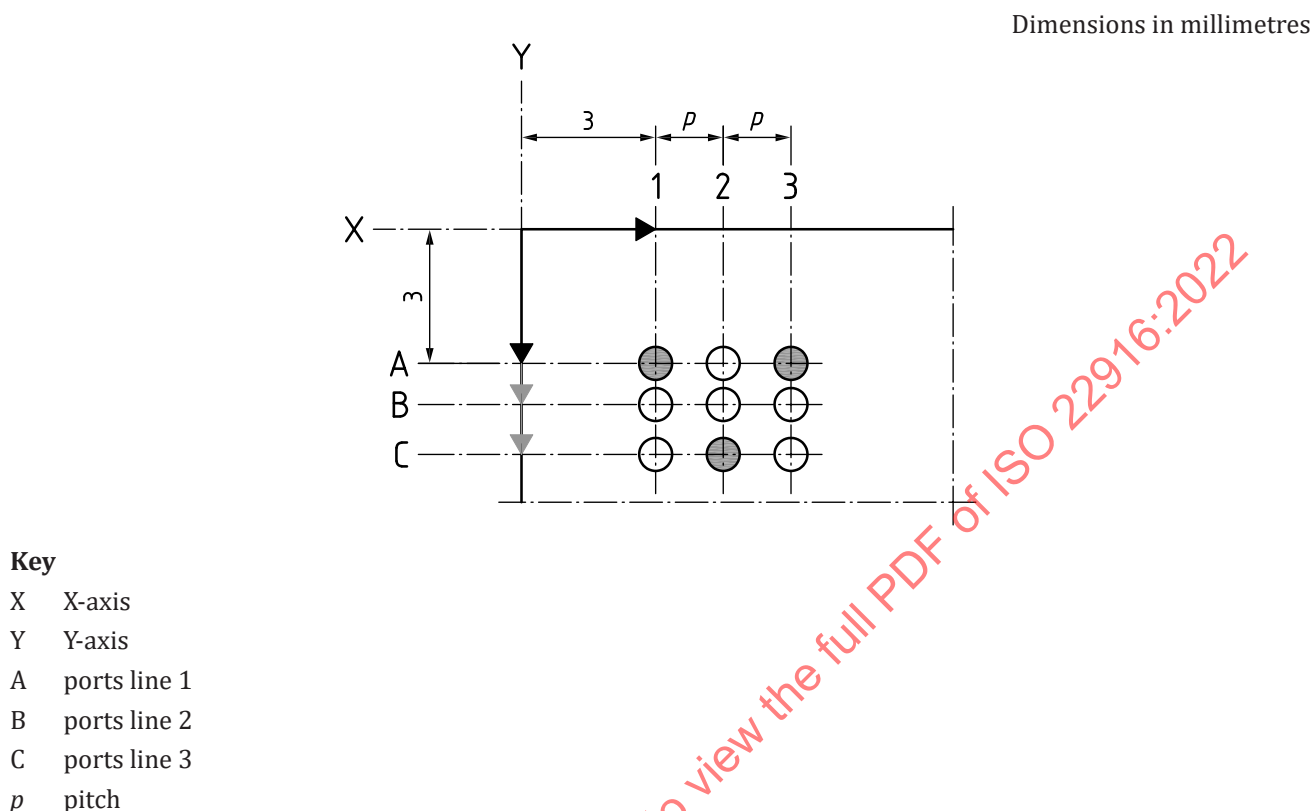
Figure 8 — Nomenclature of a microfluidic chip
