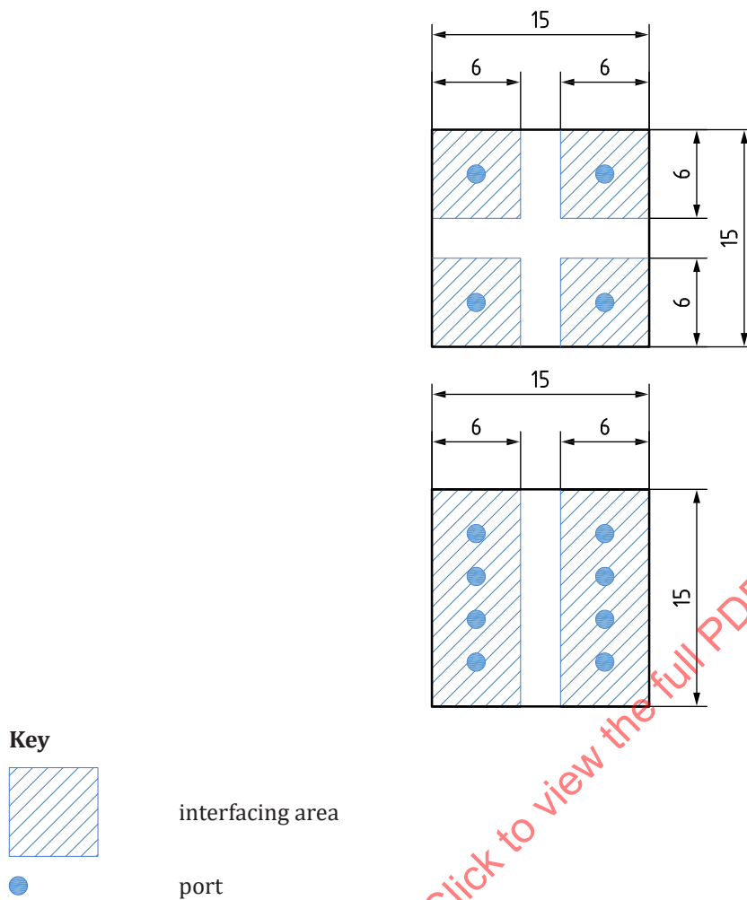
Figure 9 — Exclusion zones around portholes for a 15 mm × 15 mm chip
