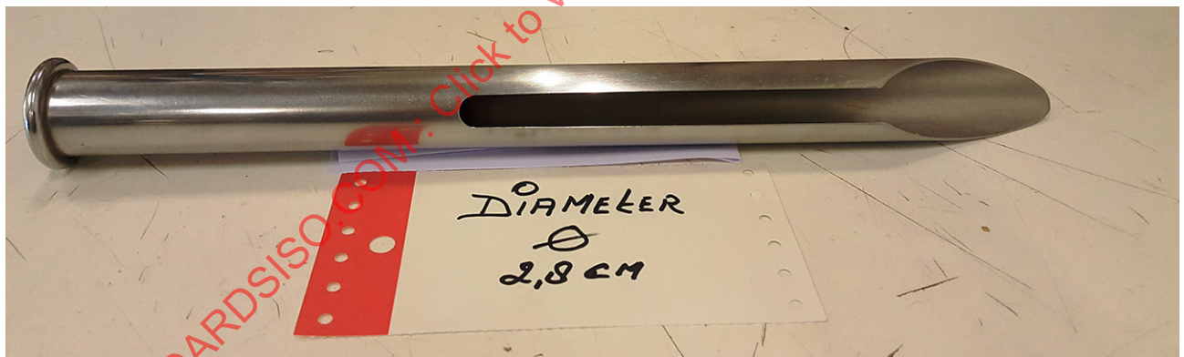
Figure A.1 — Example of a sampling spear (also known as “trier”) for sampling of bags
