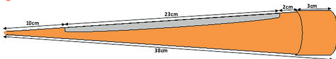
Figure A.1 — Example of a sampling spear (also known as “trier”) for sampling of bags
