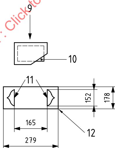
b) Details of test specimen holder
