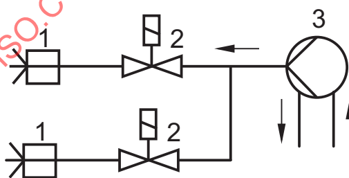
Figure F.1 — One-stage oil burners or two-stage oil burners with pressure variation (one-way or two-way systems)
