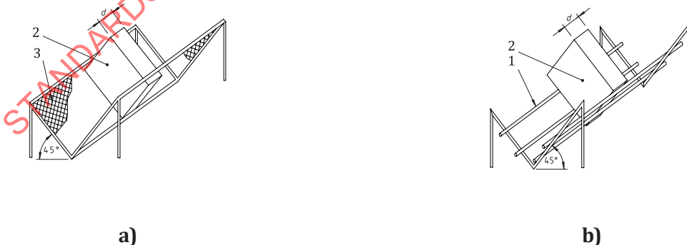
Figure 7 — Example of equipment for determination of water absorption by total immersion (Method 2C)
