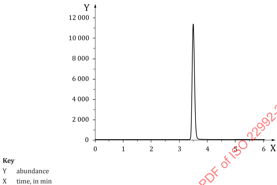
Figure A.1 — HPLC-MS/MS chromatogram of triclosan (transitions 286,7/35,0)
