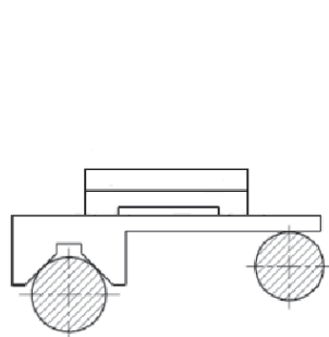
Figure 123 — Auxiliary blocks used for the measurement of parallelism error of two axes
