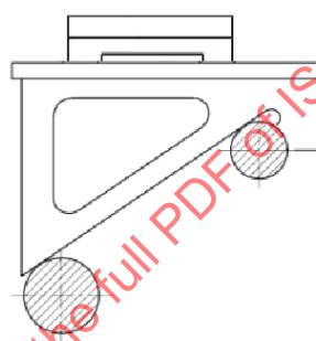
Figure 123 — Auxiliary blocks used for the measurement of parallelism error of two axes
