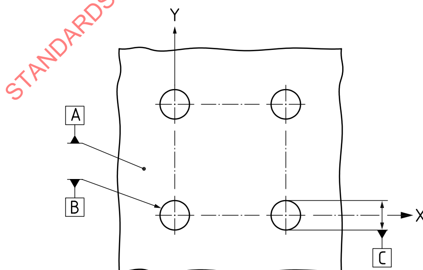
Figure 16 — Test piece with multiple holes
