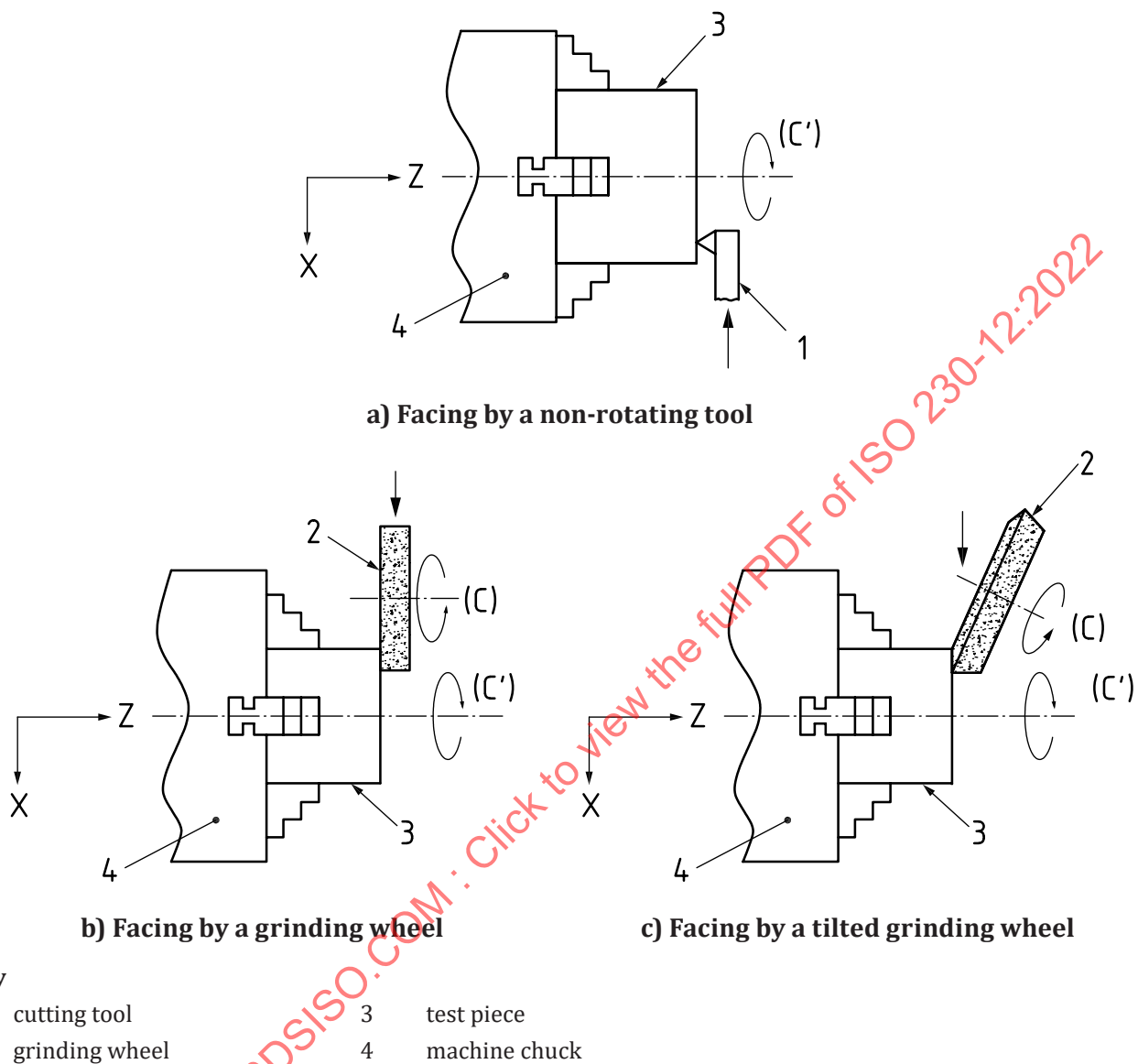
Figure 6 — Facing of a rotating test piece
