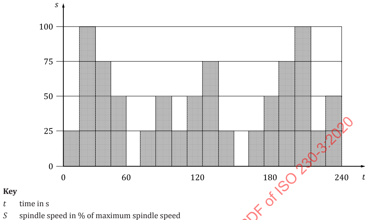
Figure 6 — Sample spindle speed spectrum for thermal distortion tests
