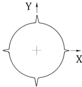
Figure B.5 — Quadrature reversal spikes
