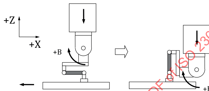
Figure C.4 — Ball bar test for circular test of X, Z and B axes in tangential direction
