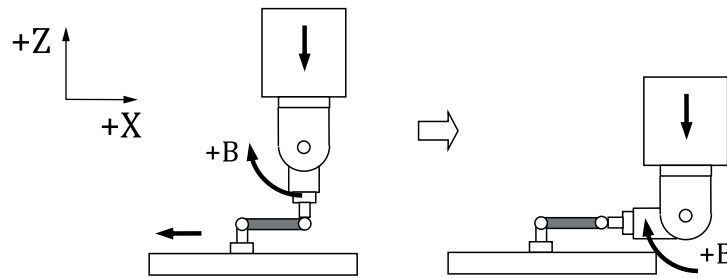
Figure C.3 — Ball bar test for circular test of X, Z and B axes in X-direction
