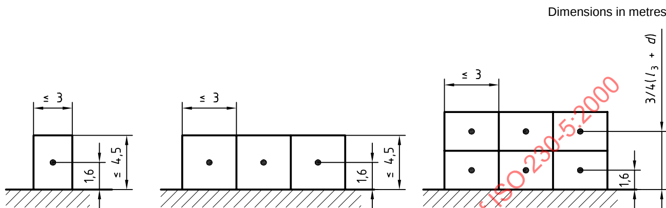
Figure A.1 — Procedure for fixing the specified microphone positions in the general case of d = 1\text{ m} (if d = 0,5\text{ m} , see ISO 3746)
