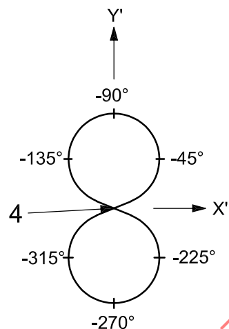
b) Enlarged end view of assumed path of axis of rotation in the X'-Y' plane
