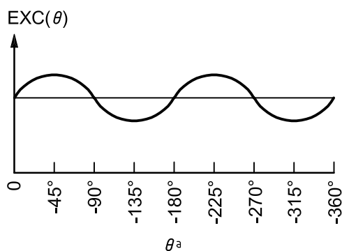
c) Rectilinear plot of radial error motion [ X' component in b) versus angle of rotation]
