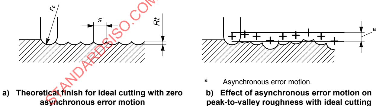
Figure A.12 — Relationship of surface roughness to asynchronous error motion
