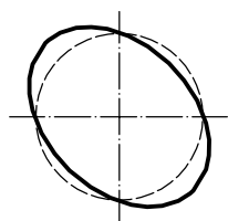
a) Radial error motion polar plot
