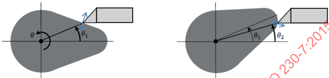
Figure 6 — Illustration of varying sensitive direction for cam turning operation
