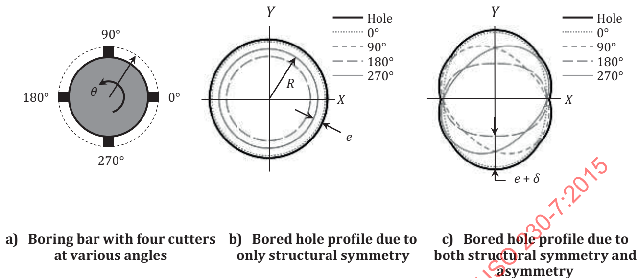
Figure A.12 — Hole profiles for multi-cutter boring bar due to structural symmetry and structural asymmetry
