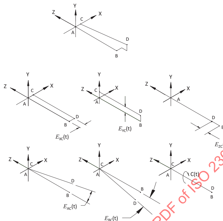
a) Schematic diagrams of general relative motion and six basic degrees of freedom between axis average line and axis of rotation at time, t
