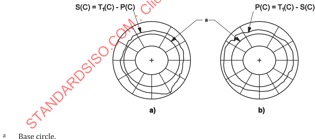
Figure B.3 — Error separation by profile subtraction using data of Figure B.2
