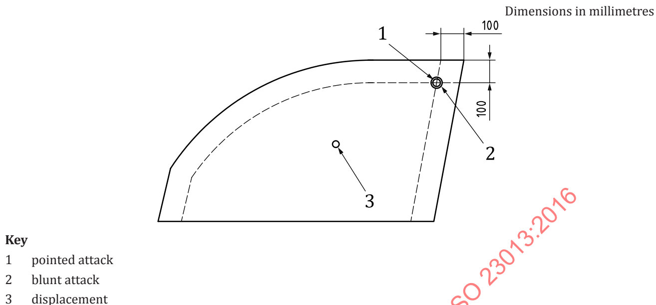
Figure 8 — Top corner test position for attack sequence with blunt tool, taking a front door window as an example
