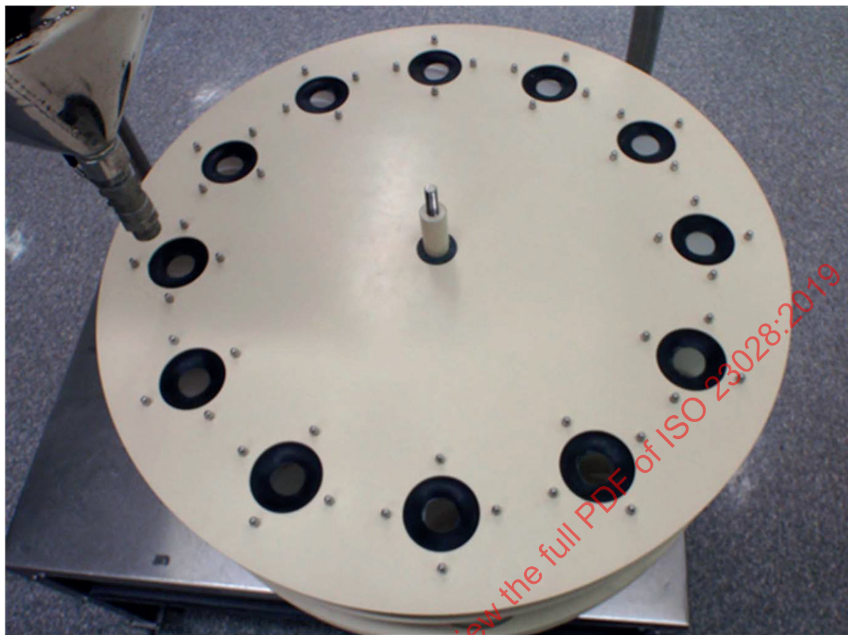
Figure A.2 — Plate that fits over receiver containers with rubber seals to prevent fines loss while splitting is in progress
