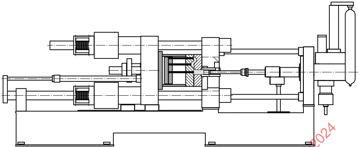
Figure A.3 — Example of a horizontal cold-chamber die casting machine with a toggle free die closing system
