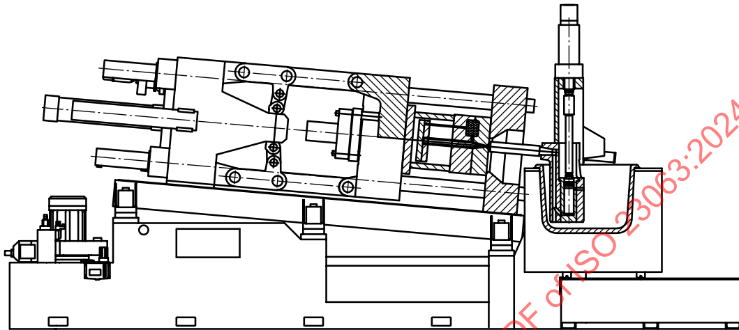
Figure A.1 — Example of a hot-chamber die casting machine
