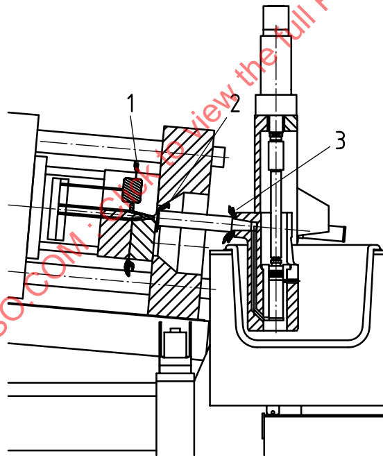
Figure A.5 — Examples of danger zones for metal spraying at horizontal cold-chamber die casting machines
