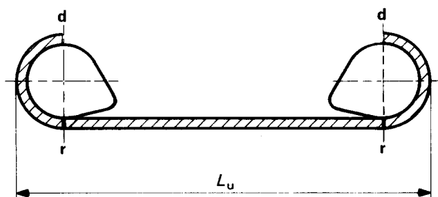
FIGURE 3 — Test piece mounted on pulleys ("cors de chasse")
