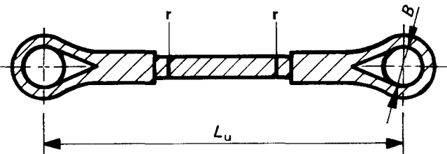
The limiting marks "r" shall be 150 mm from the last turn of the splice.
