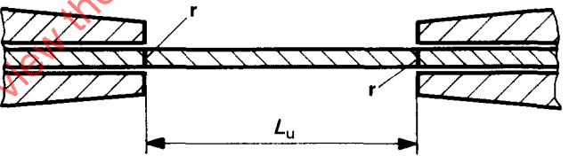
The limiting marks "r" of the test piece shall be positioned in line with the grips.
