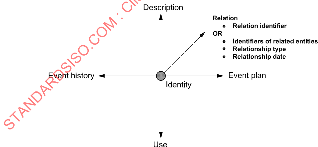
Figure 15 — Relation metadata
