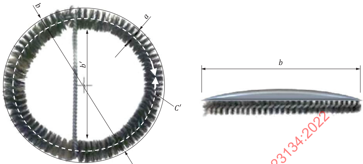
Figure E.2 — Dimensions of the tube brush and cap
