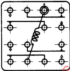
Circuit diagram of the base connections
