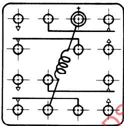
Circuit diagram of the base connections
