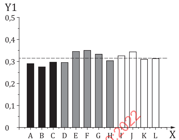
b) Concentration result of 7 nm HfO 2 sample by using newly fitted electronic stopping power
