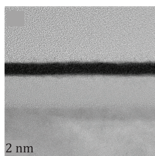
c) 5 nm HfO 2 on a 12 nm thermal SiO 2 /Si substrate
