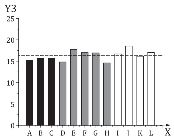
f) Quantity of Hf of 7 nm HfO 2 sample by using newly fitted electronic stopping power
