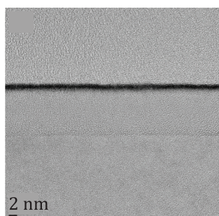
a) 1 nm HfO 2 on a 12 nm thermal SiO 2 /Si substrate
