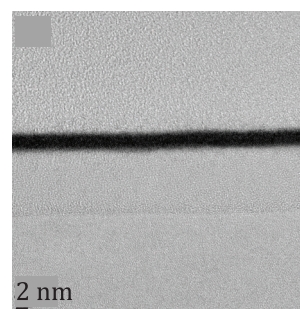
b) 3 nm HfO 2 on a 12 nm thermal SiO 2 /Si substrate
