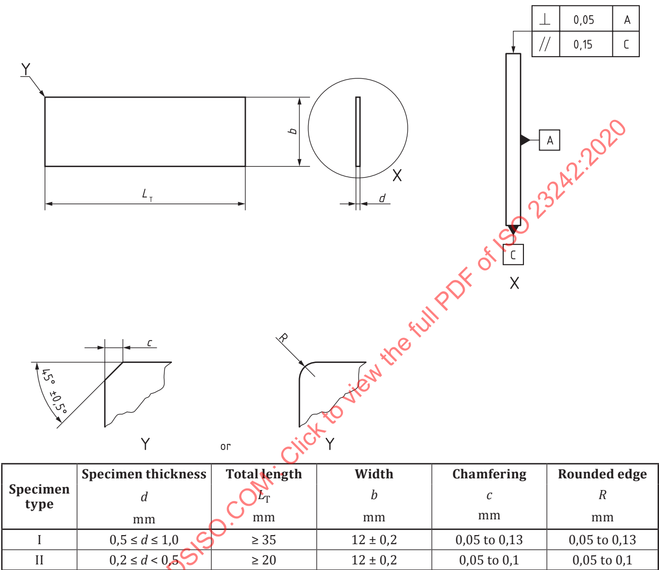
Figure 3 — Dimensions of specimen
