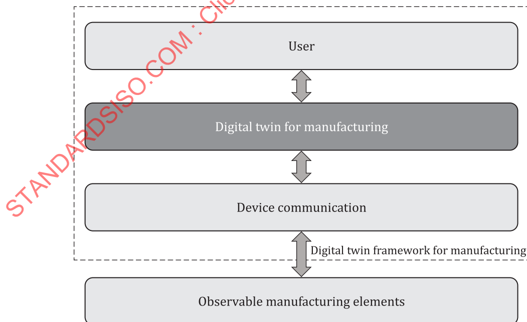
Figure 3 — Boundary of the digital twin framework for manufacturing
