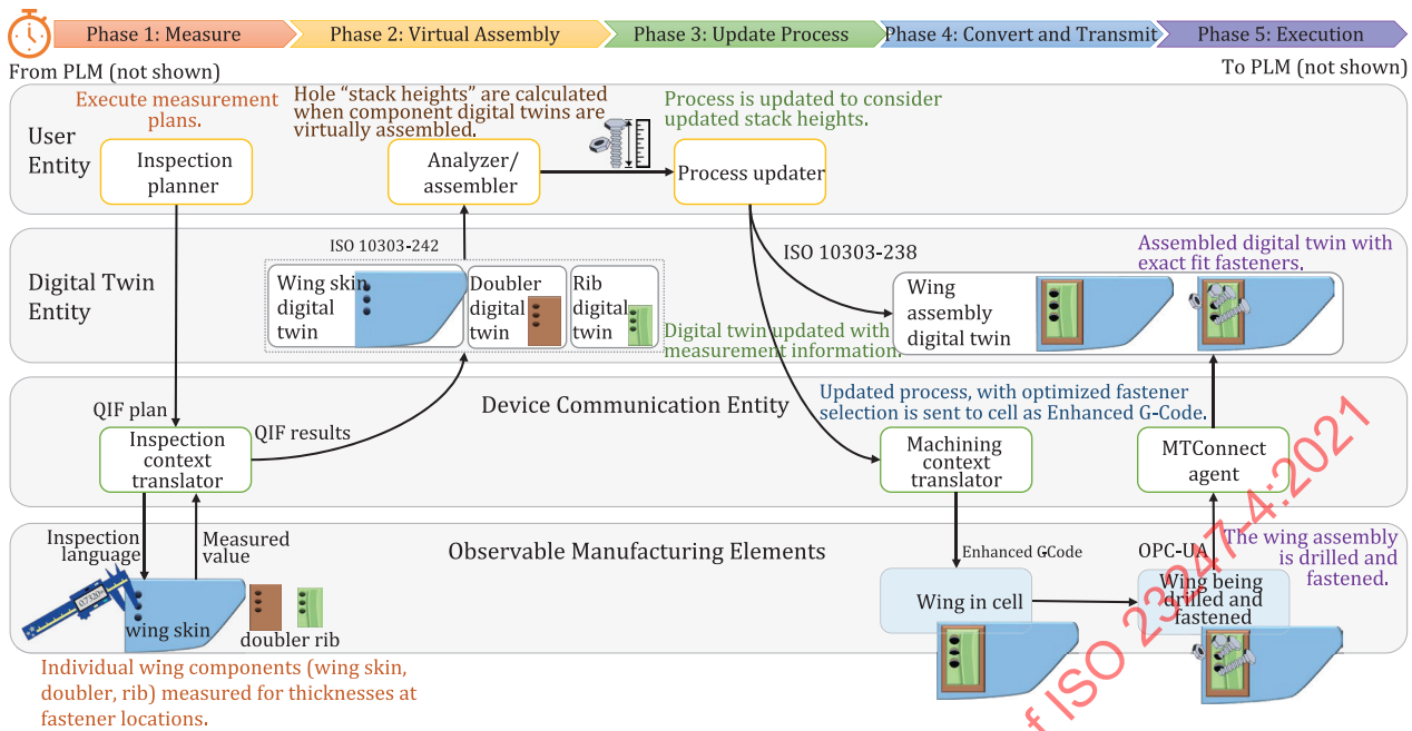
Figure C.1 — Process flow of advanced metrology
