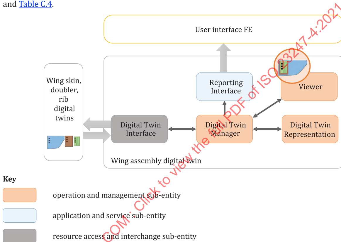
Figure C.4 — Implementation mapping of wing assembly digital twin to digital twin entity
