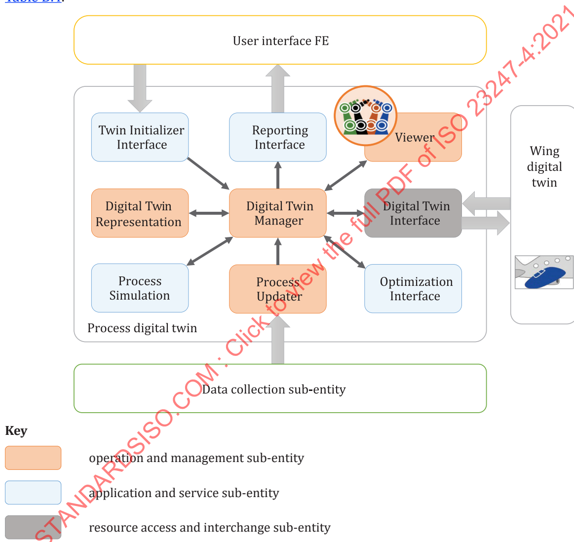
Figure B.4 — Implementation mapping of process digital twin to digital twin entity
