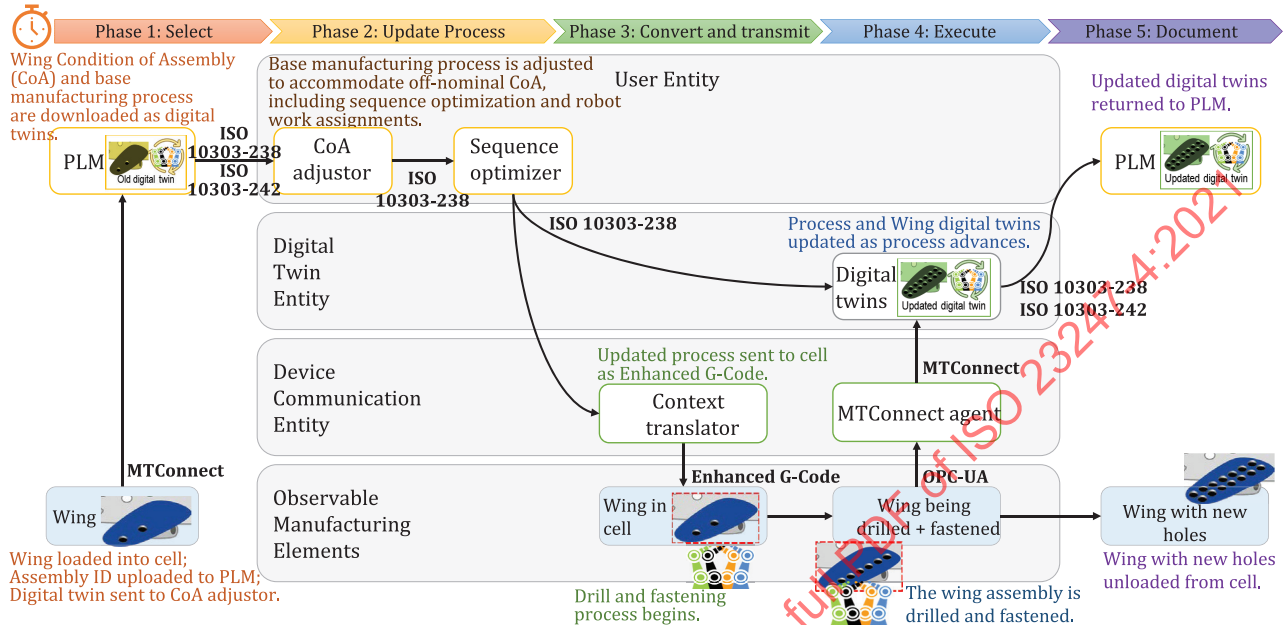
Figure B.1 — Process flow of dynamic scheduling
